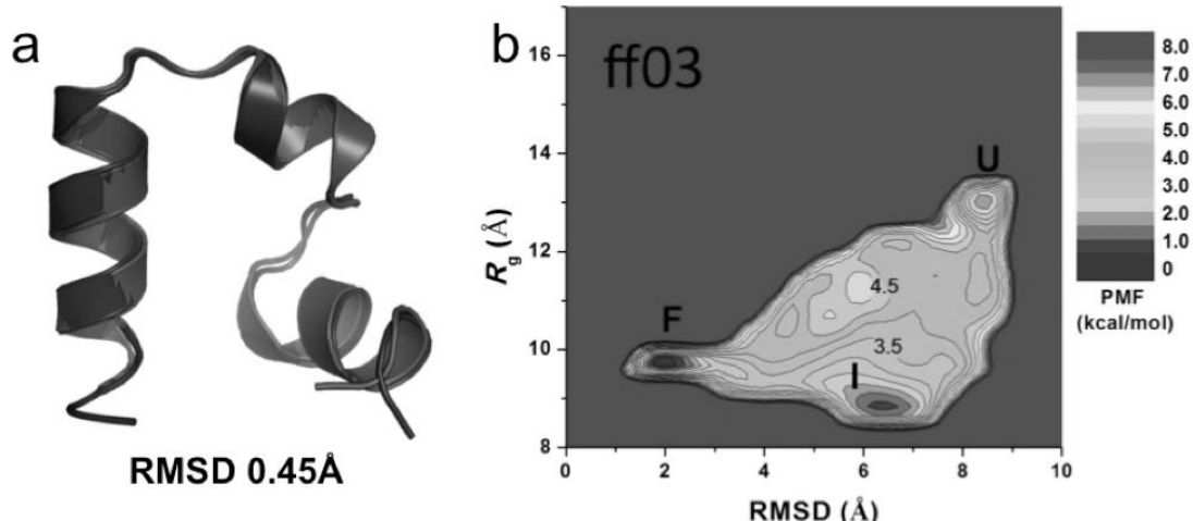
Figure 1. Folding of wild-type villin simulated via aMD: (a) comparison of simulation-folded villin (blue) with the PDB (1YRF) native structure (red) (b) two-dimensional (RMSD, R_g ) free energy profiles calculated by reweighting the aMD simulations.
